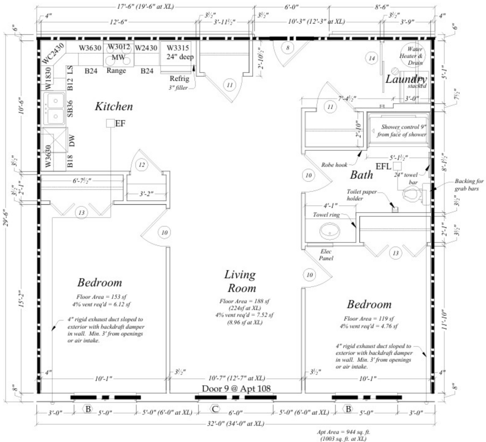
2 Bedroom #2 Layout Scale: 1/4" = 1'-0"
